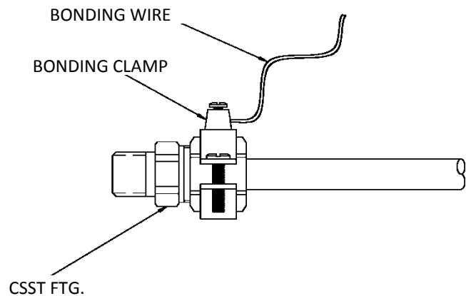
Figure 2: Bonding Clamp on CSST Fitting
